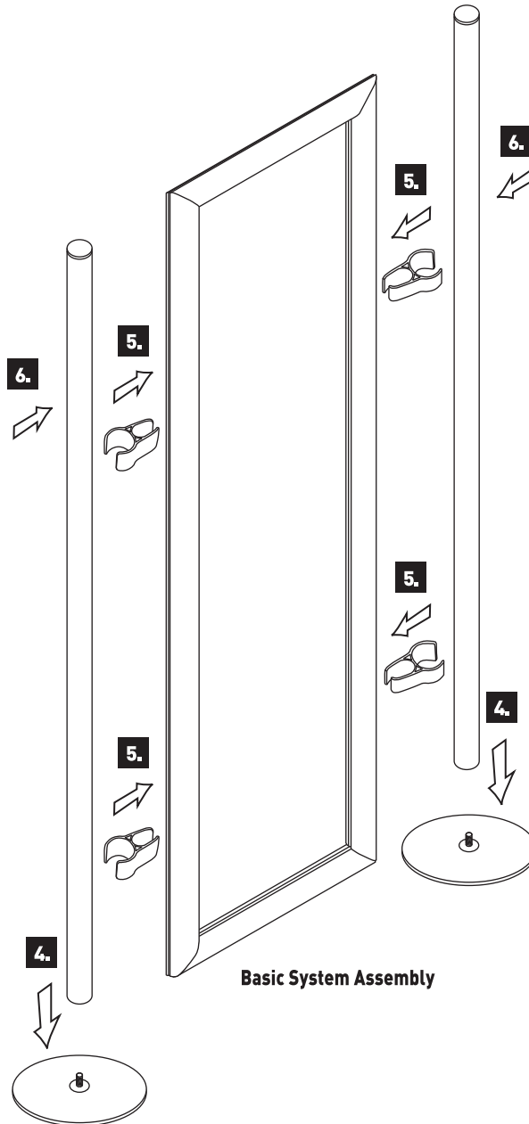
SnapOn Clip™
